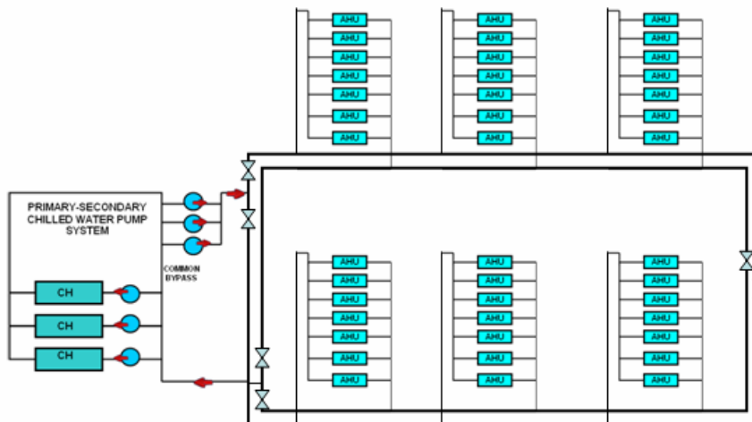
Figure 5: Primary/Secondary chilled water distribution system with reverse return and ring loop piping
