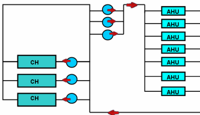
Figure 5: Primary/Secondary chilled water distribution system with reverse return and ring loop piping
