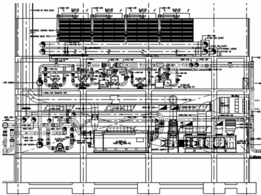
Fig 7 : Chiller plant design with individual companion pump and short run to minimize system friction loss
