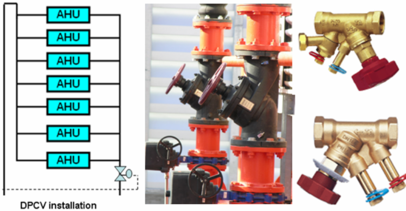
Fig 6 : Balancing valve and DPCV is the effective tool of system balancing
